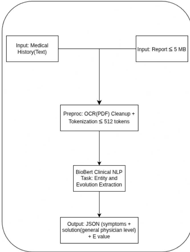
Fig. 6: Stage 5 (MedProc): extraction of Evolution (E) and clinical features from patient history and reports.
