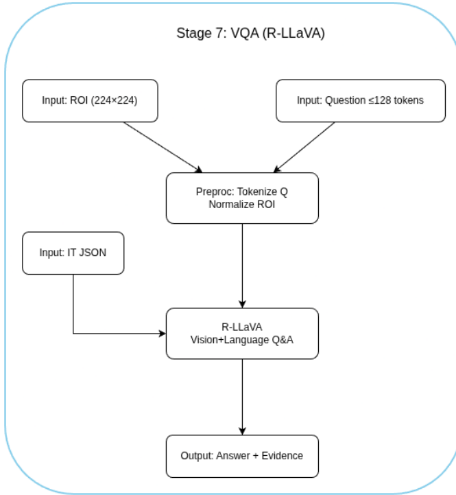
Fig. 8: Stage 7 (VQA): dermatology-focused vision–language model answering patient and clinician questions using the unified JSON and lesion imagery.
