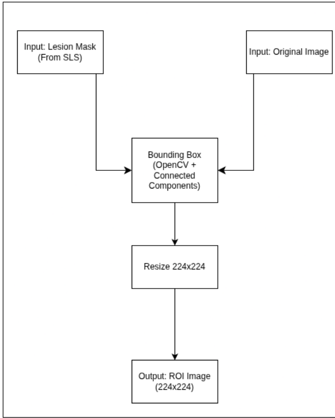
Fig. 4: Stage 3 (SLRC): mask-aware ROI cropping and normalization for classification.
