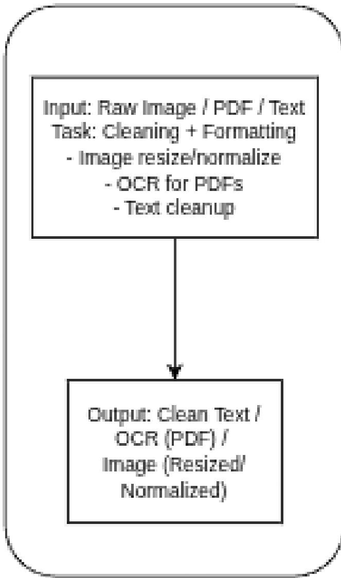
Fig. 2: Preprocessing stage: unifying image and text inputs into standardized training-ready and inference-ready formats.
