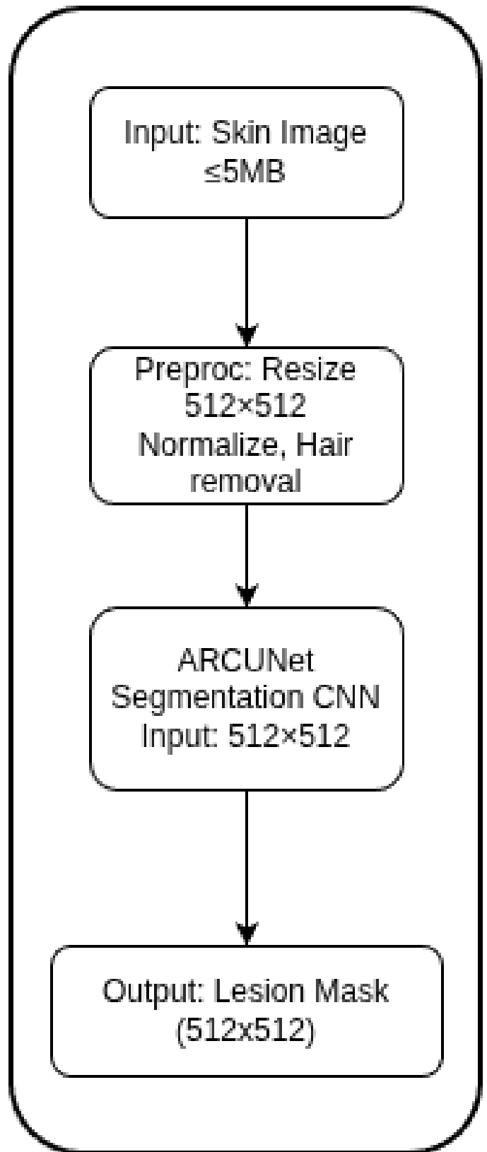
Fig. 3: Stage 2 (SLS): segmentation of lesion area and extraction of geometric mask descriptors.
