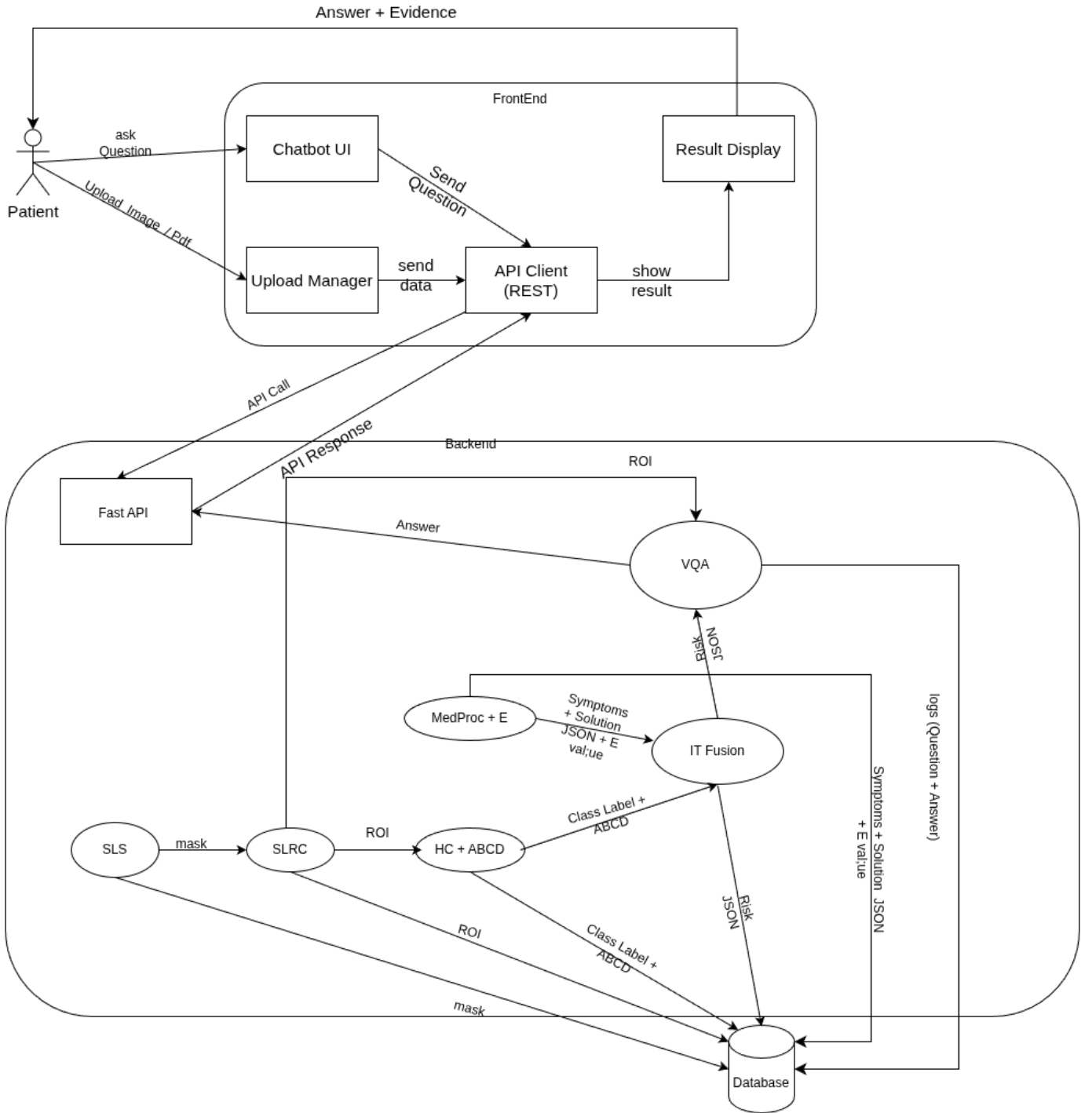
Fig. 1: High-level NutriDermAI architecture: staged pipeline from raw patient inputs to ABCDE-aware risk assessment and VQA.
